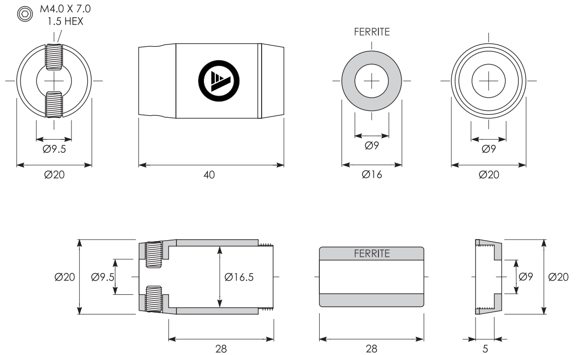
TECHNICAL VIEW
